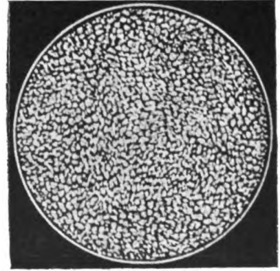
Fig. 3—Magnified surface of polished manganese bronze after being etched with dilute nitric acid. Magnified 48 diameters
